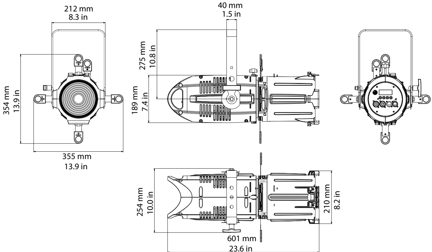
Reflection LEDko with optic Soft Profile Fresnel
