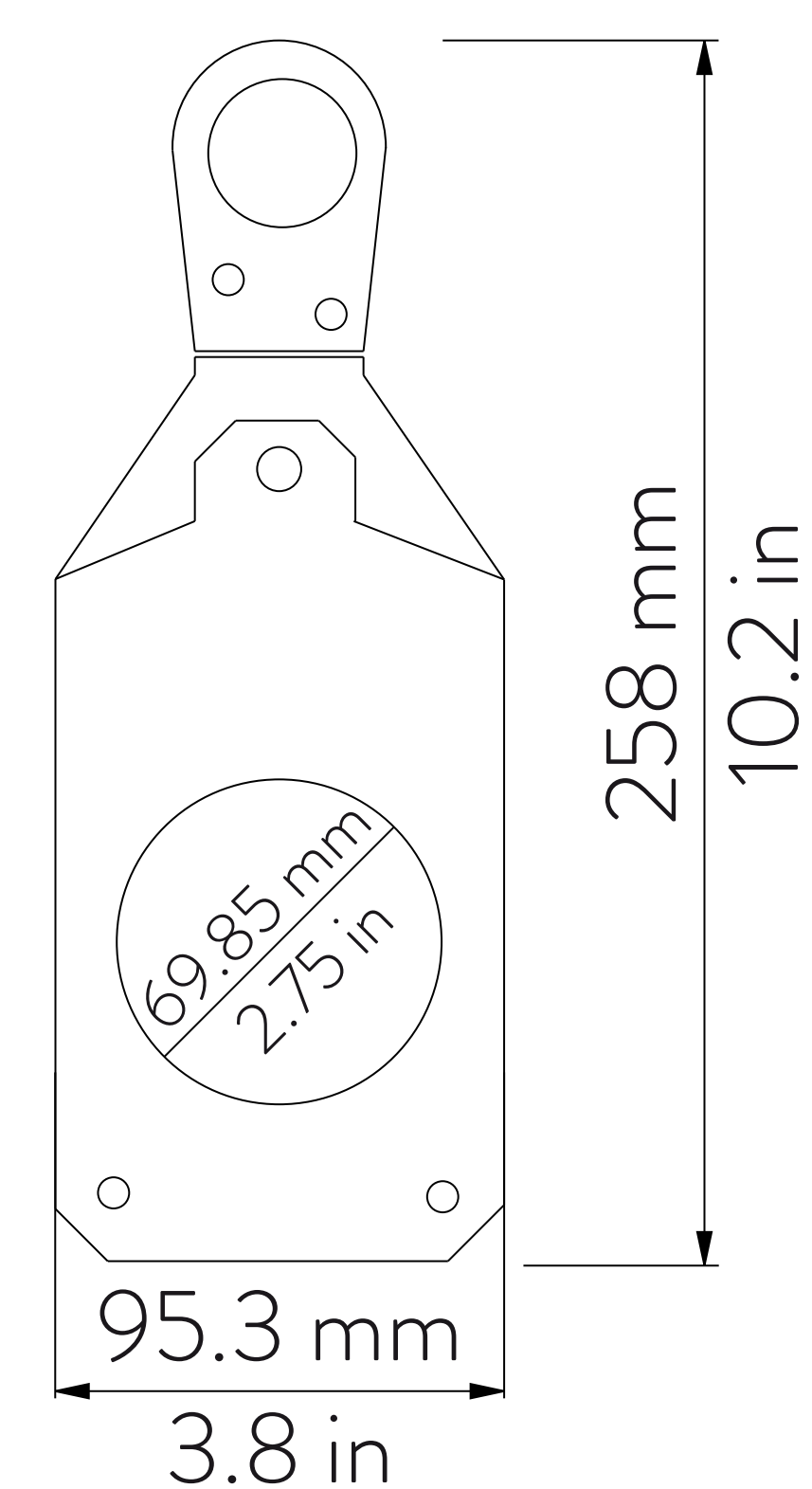
Gobo holder for glass gobo
