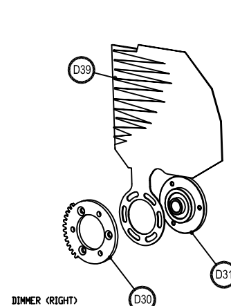
DIMMER (RIGHT)
