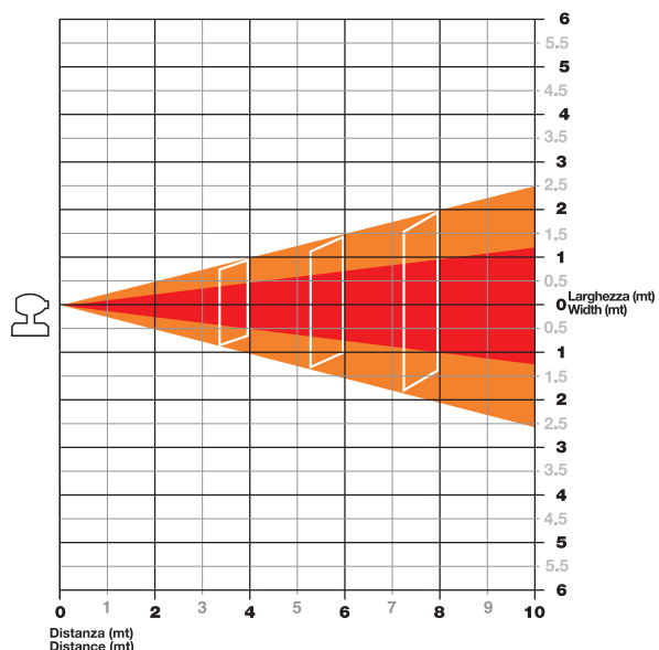
Horizontal Beam
