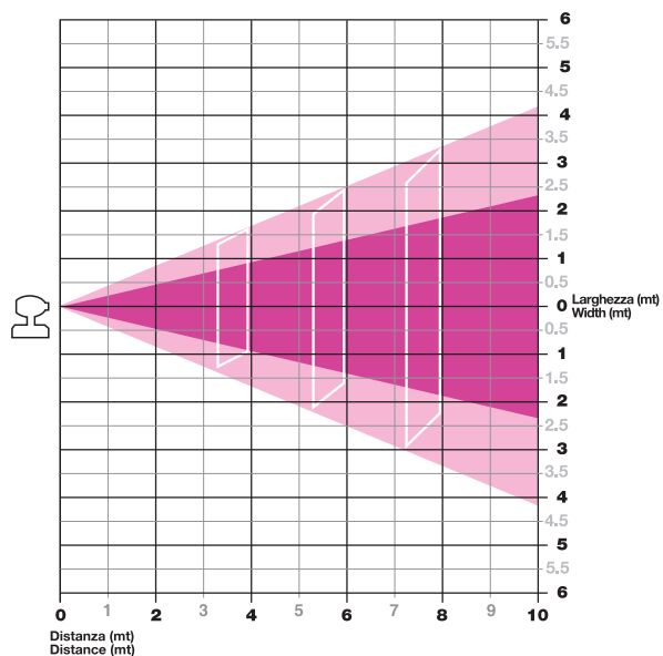
Horizontal Beam
