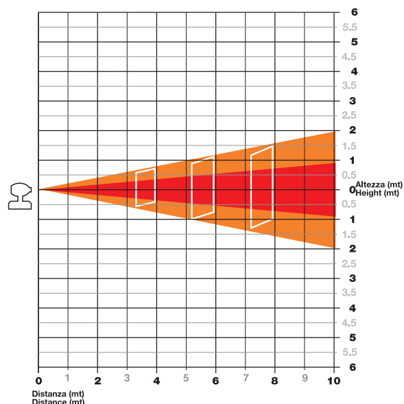
Vertical Beam
