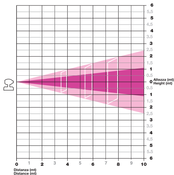
Vertical Beam
