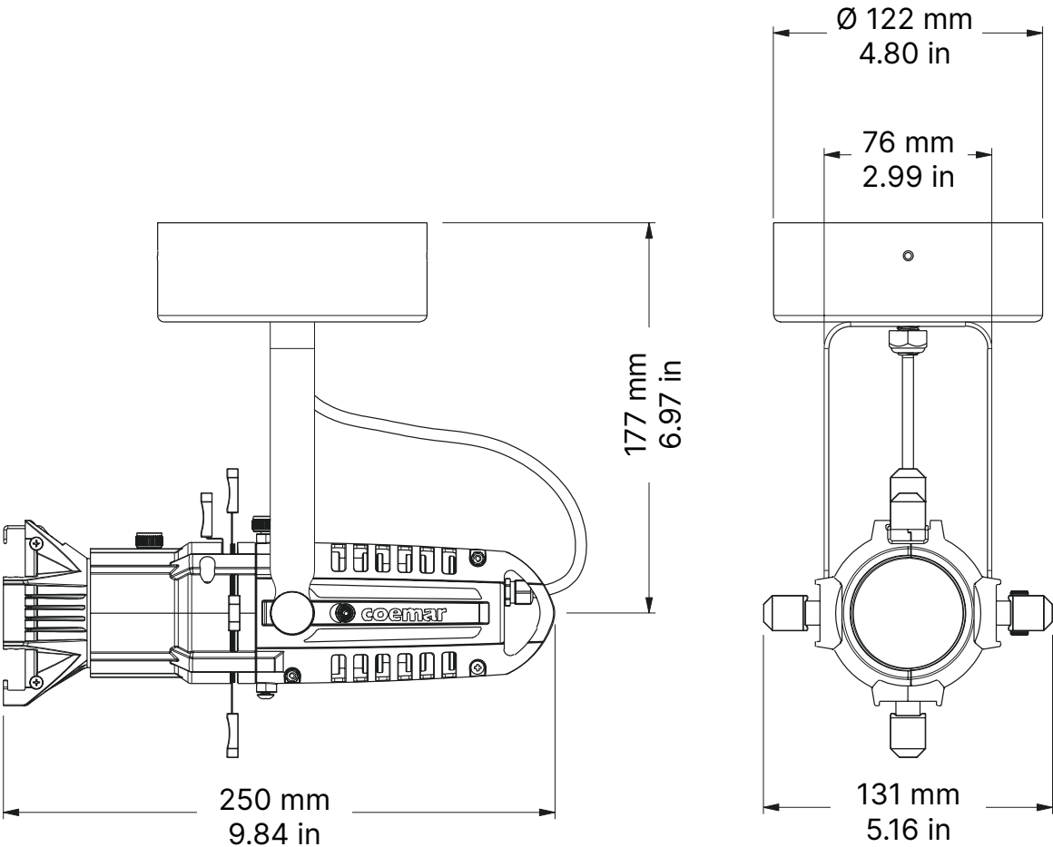
Canopy version
