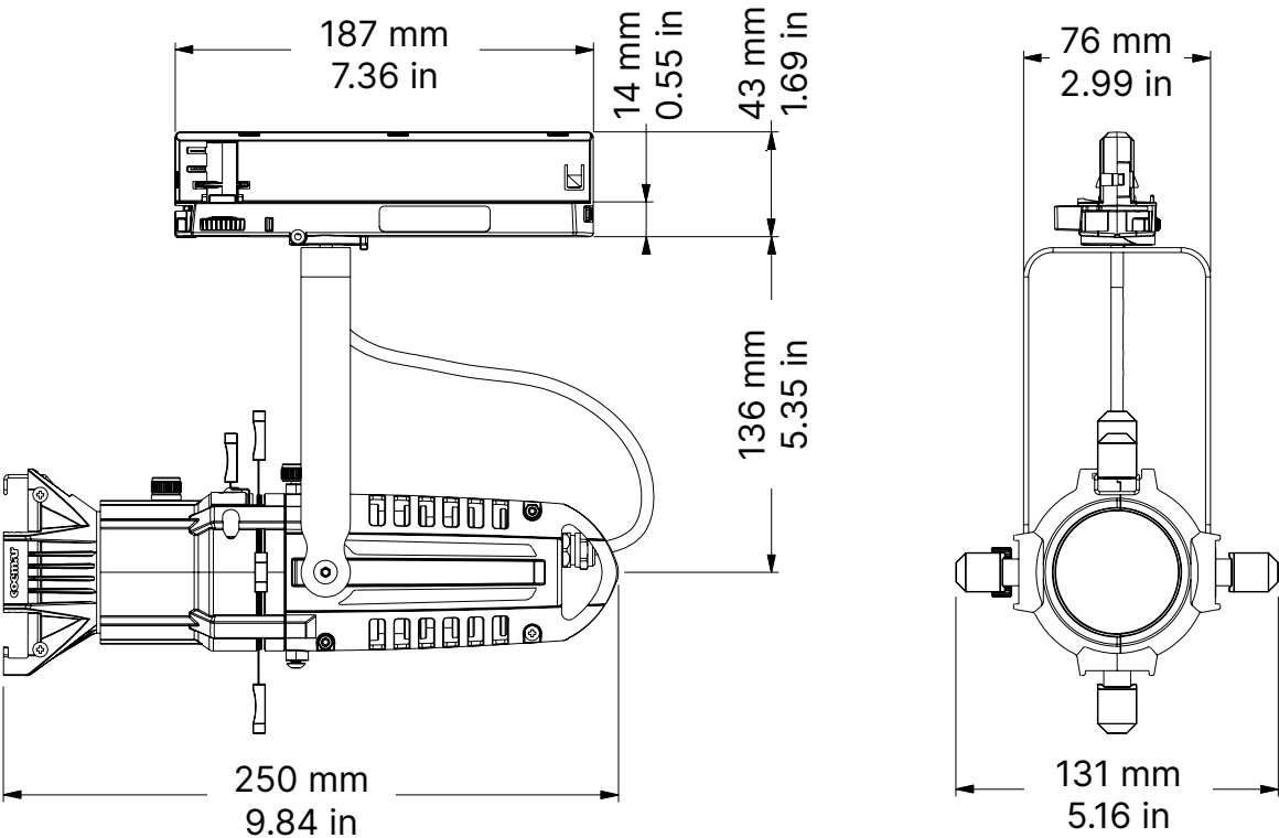
Track version with potentiometer on-board
