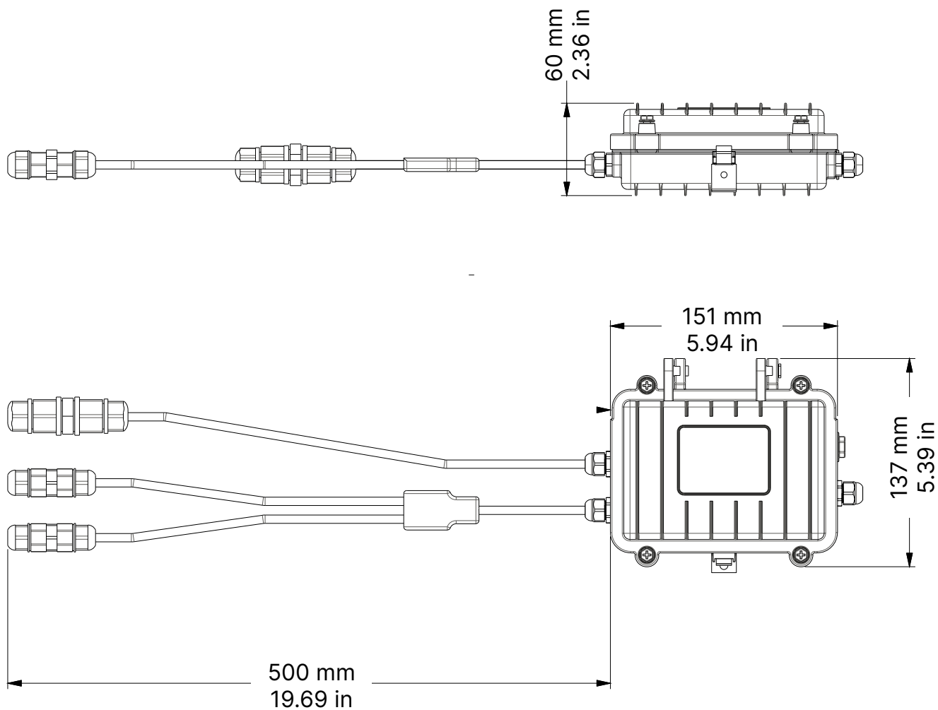
Portable version
